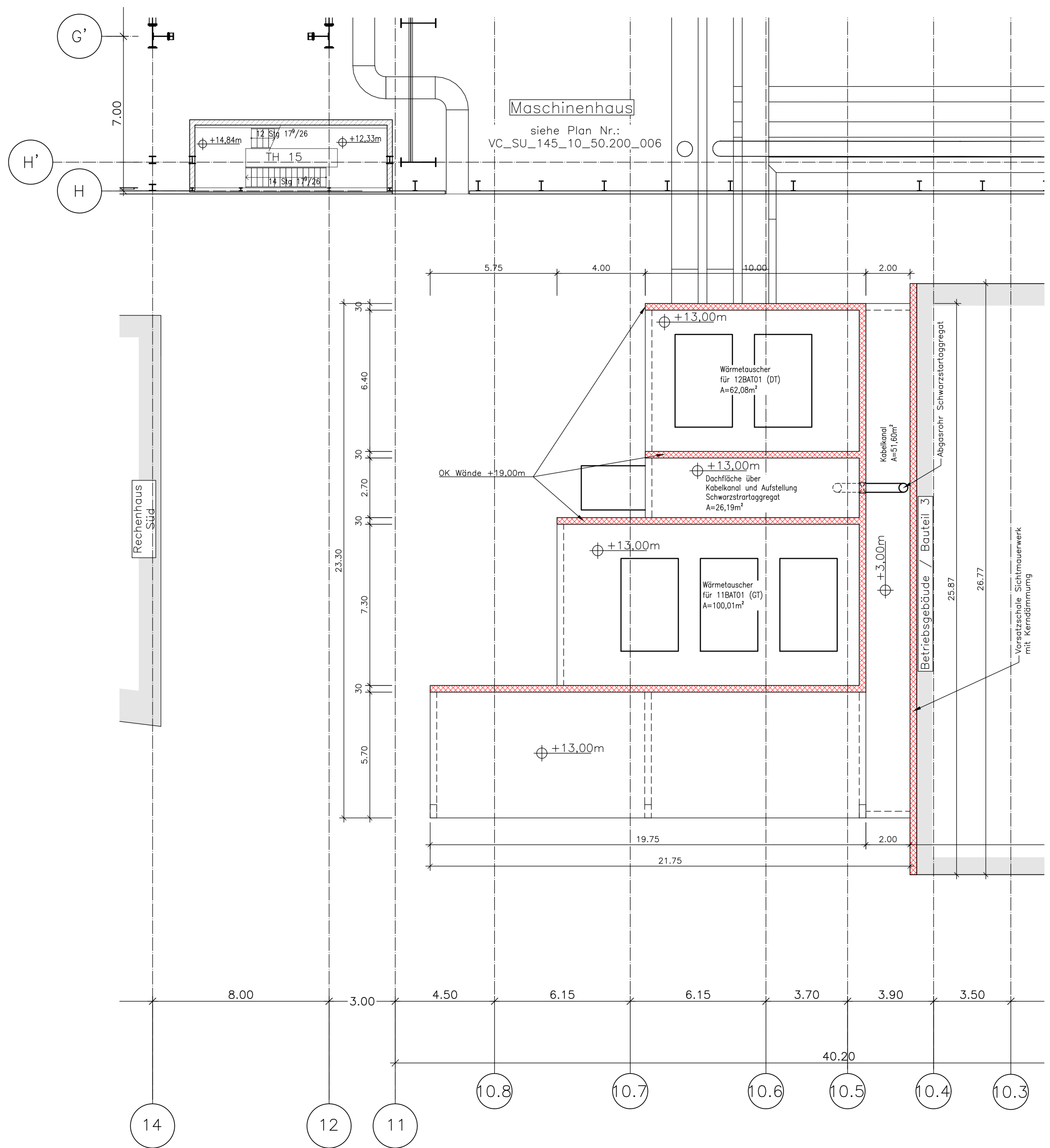
Grundriss +13,00m (Trafos) M 1:100
