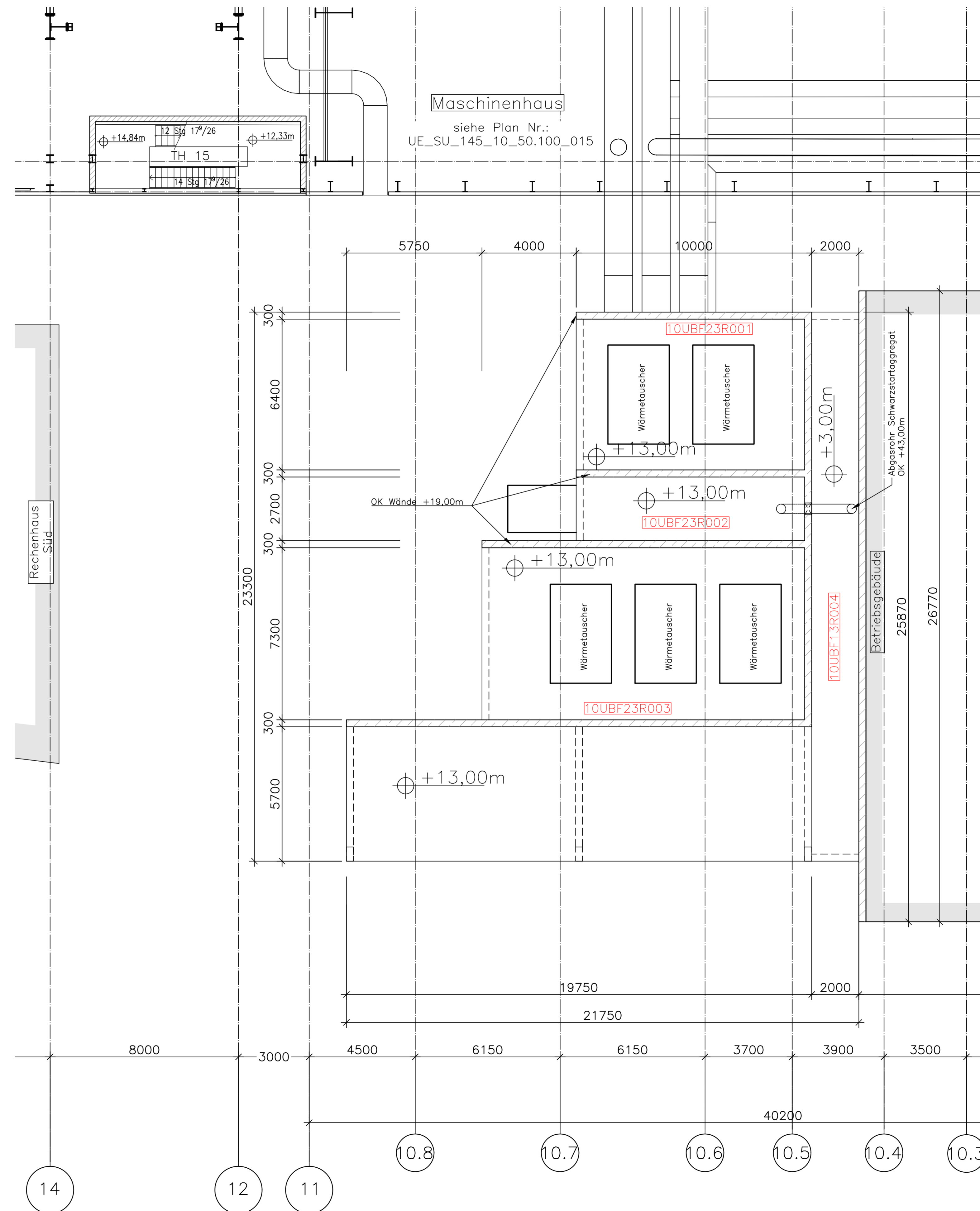
Grundriss +13,00m (Trafos) M 1:100
