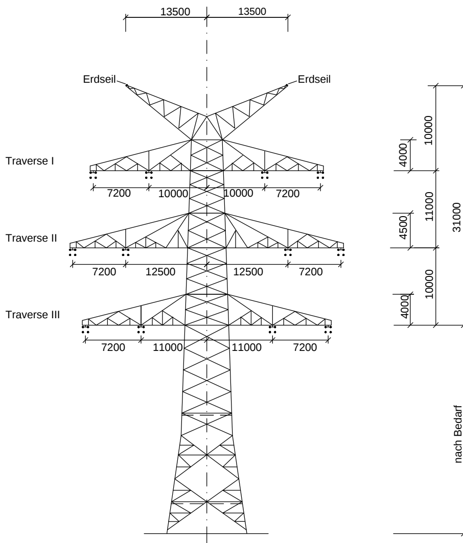
Winkelabspannmast WA120; DD-4-TT-2015.1 Ltg. Nr. 315: Mast-Nr. 54, 55, 57
