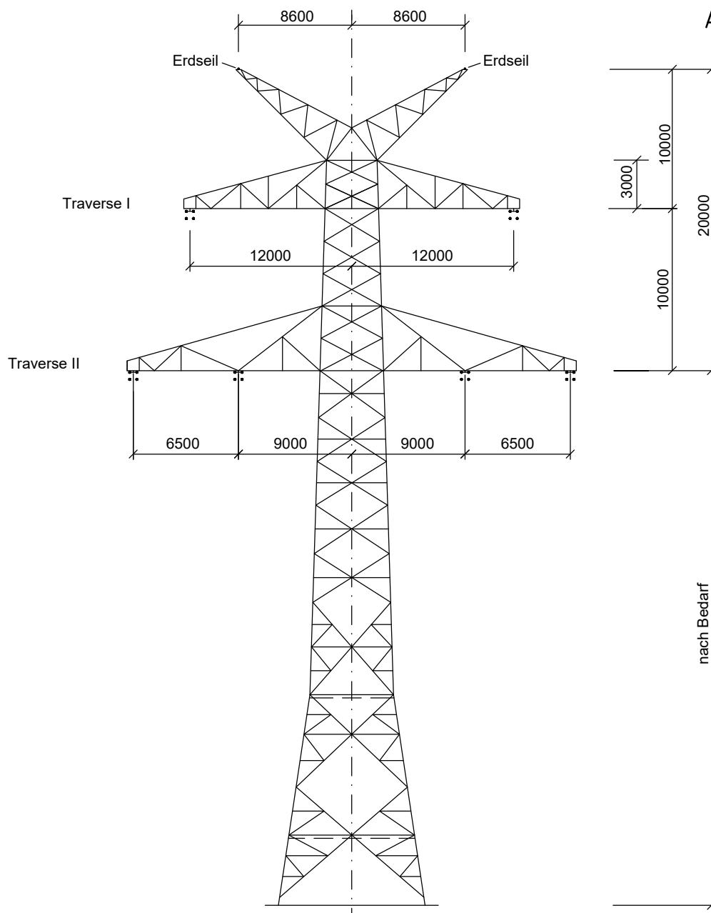
Winkelabspannmast WA140; D-2-D-2015.3 Ltg. Nr. 315: Mast-Nr. 2, 8, 9, 20, 23, 24, 26, 28 , 34, 41
