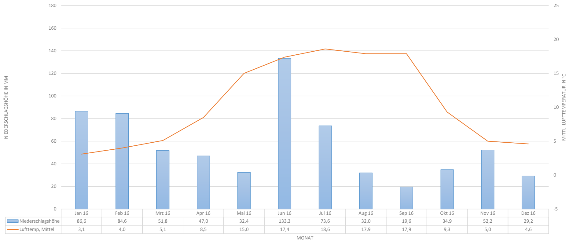
Klimadaten 2016, Station Lingen
