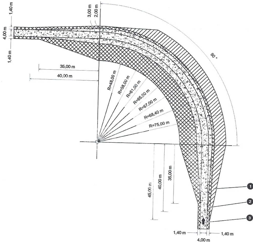
Abb. 2: Kurvenradius 90 Grad
